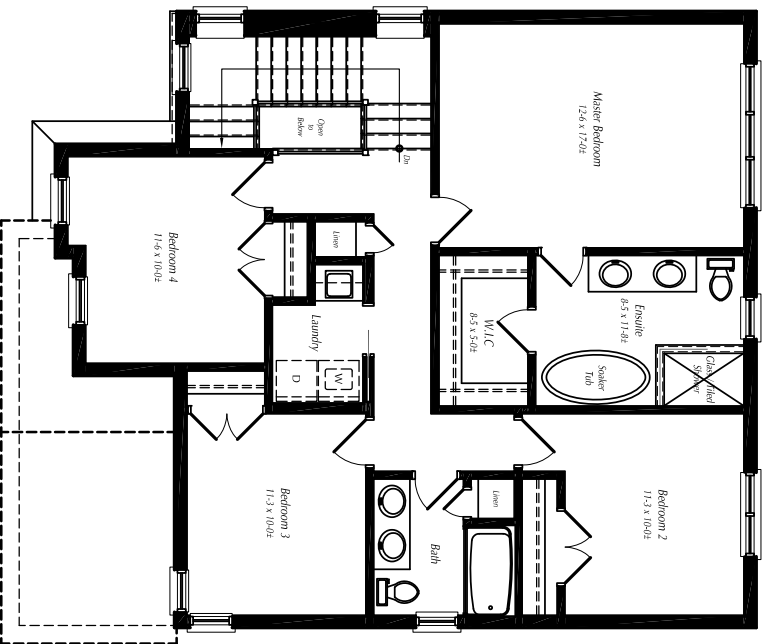
Second Floor Plan (1152 sq.ft.) (Plus 15 sq.ft. Open Space)
