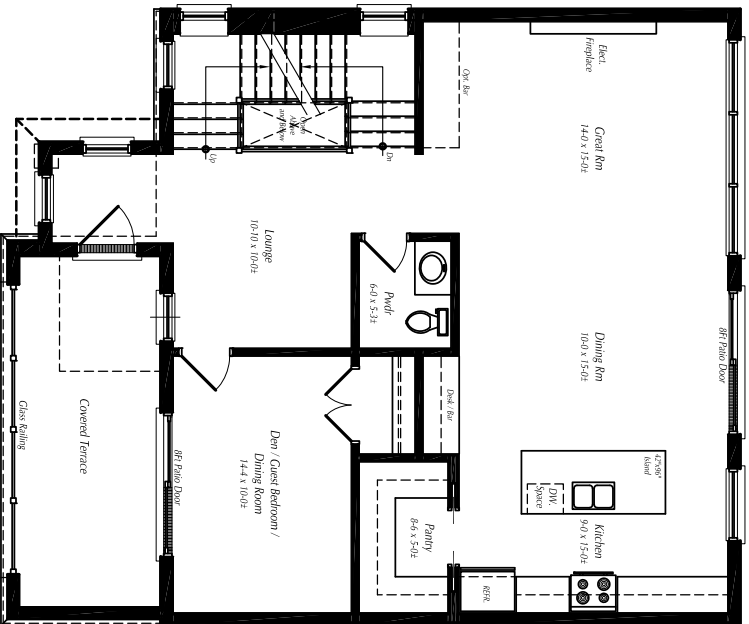
Main Floor Plan (1113 sq.ft.) (Plus 15 sq.ft. Open Space)
