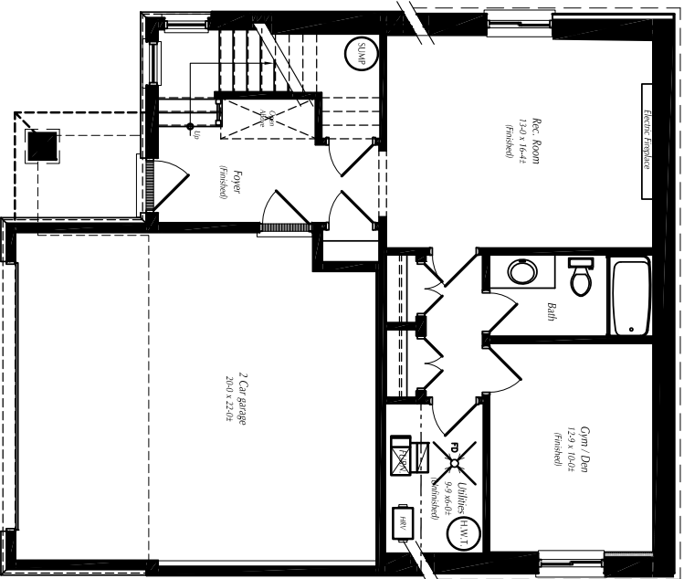
Basement / Foundation Plan (598 sq.ft. Finished)
